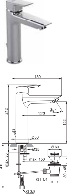
Tesi Grand Basin Mixer A6563AA
