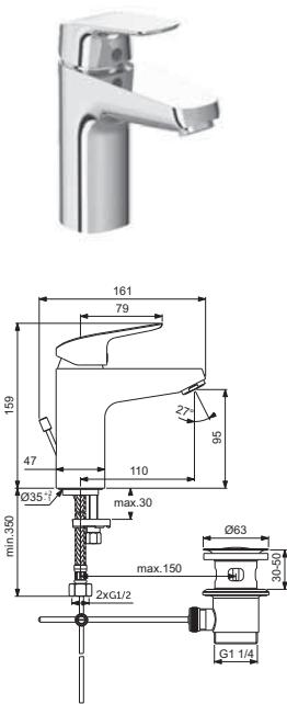
New Ceraflex Grand Basin Mixer B1713AA
