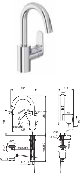
New Ceraflex High Tubular Spout Basin Mixer BC953AA
