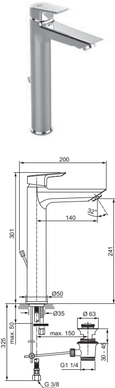
Tesi Vessel Mixer A6573AA
