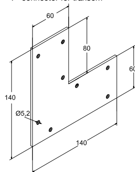
272-258 Σύνδεσμος "Γ" τεγίδων "Γ" connector for transom
