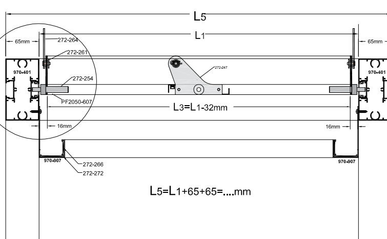
VIEW- A
